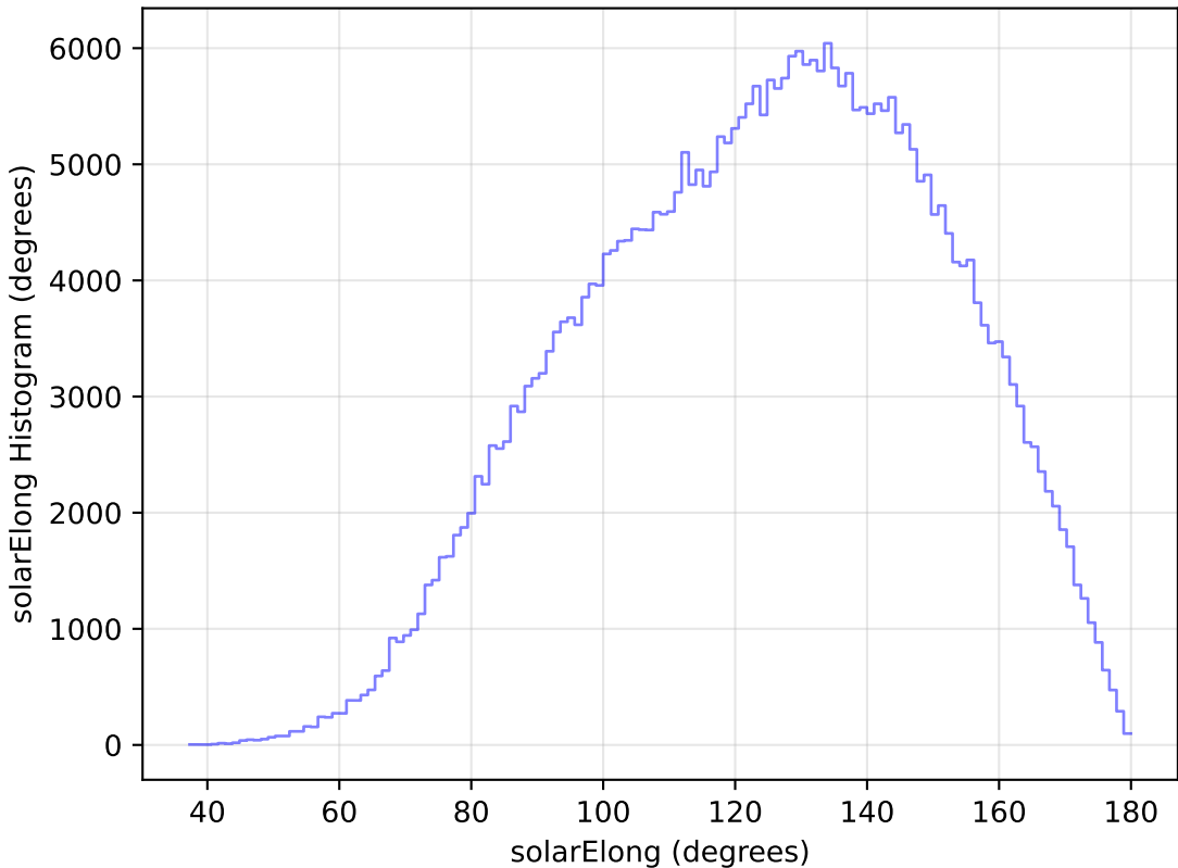
too_elab_heavy_r32_d3_gz_v3.4_10yrs WFD y band: solarElong Histogram
