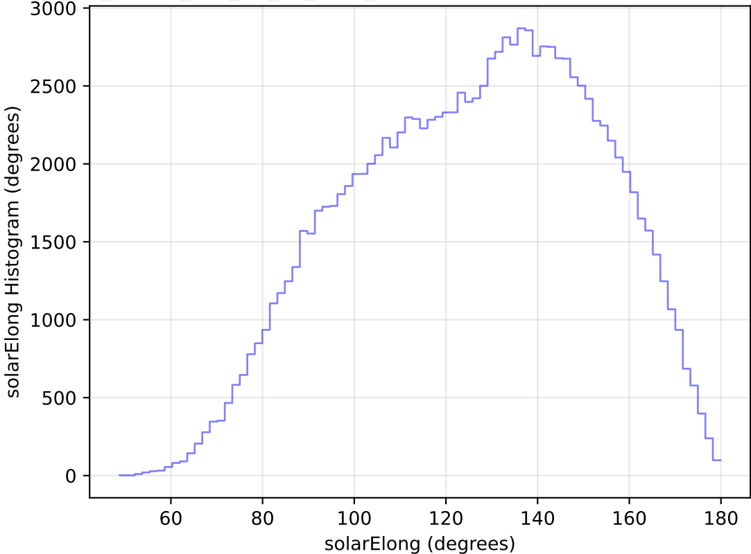
too_elab_heavy_r32_d3_gz_v3.4_10yrs WFD u band: solarElong Histogram
