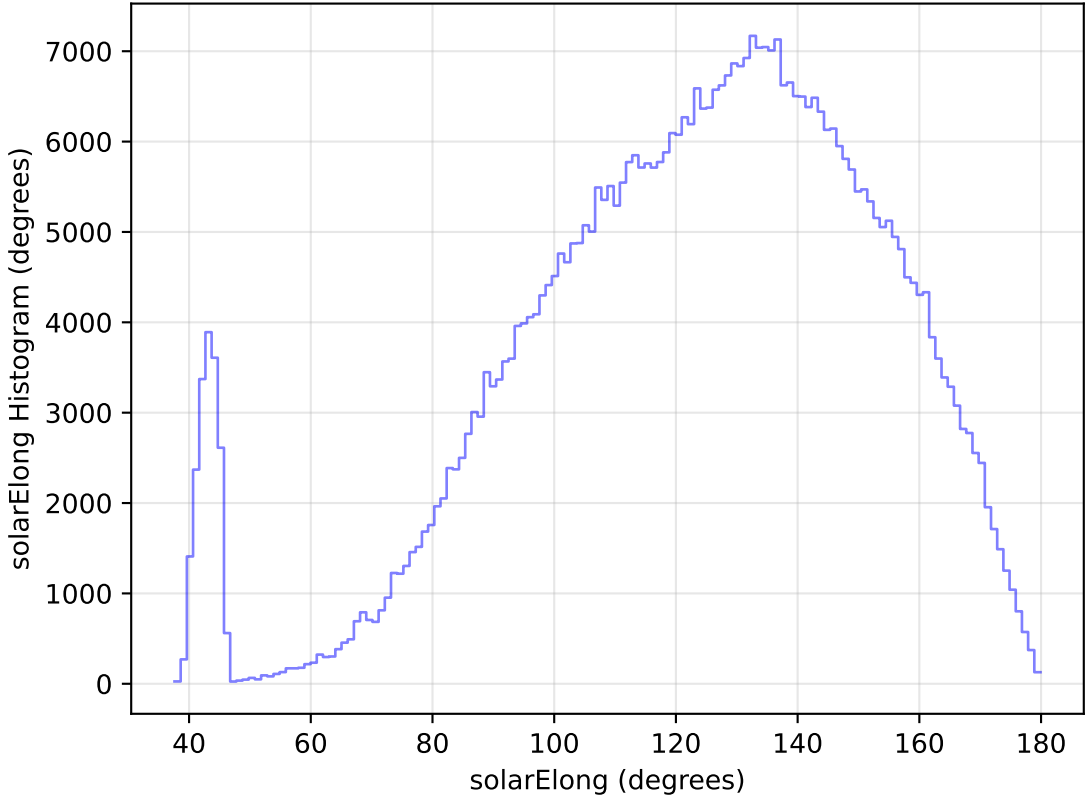
too_elab_heavy_r32_d3_gz_v3.4_10yrs WFD r band: solarElong Histogram
