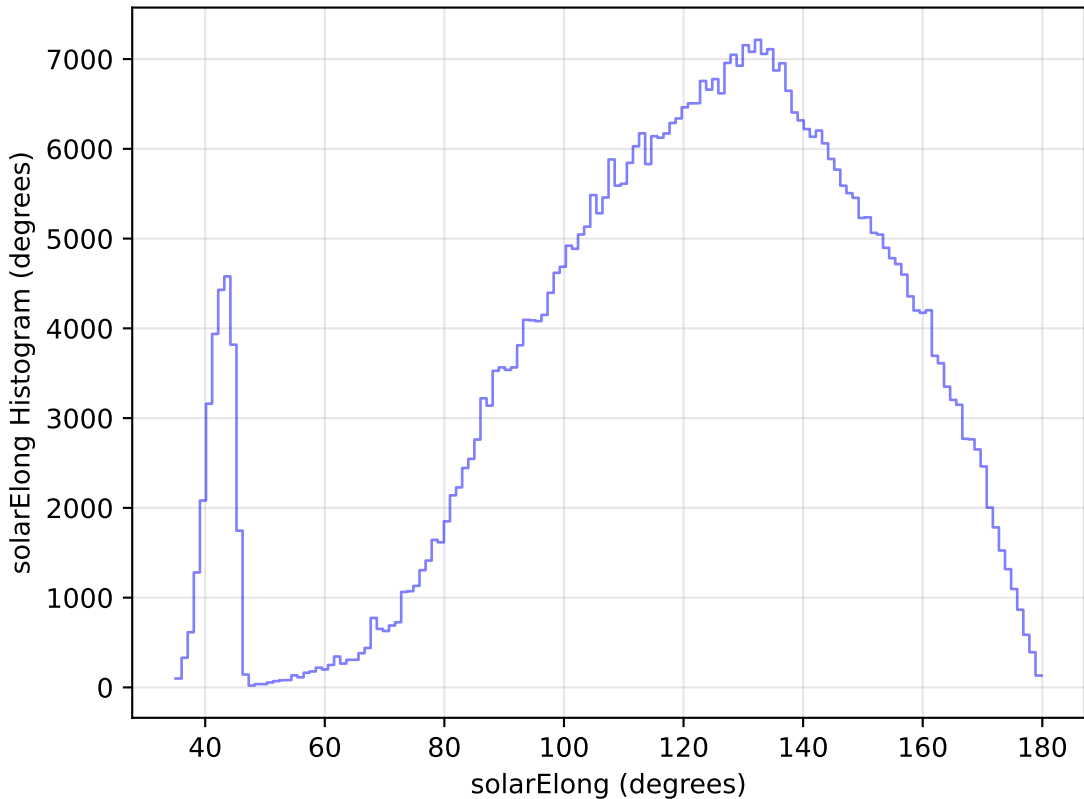
too_elab_heavy_r32_d3_gz_v3.4_10yrs WFD i band: solarElong Histogram
