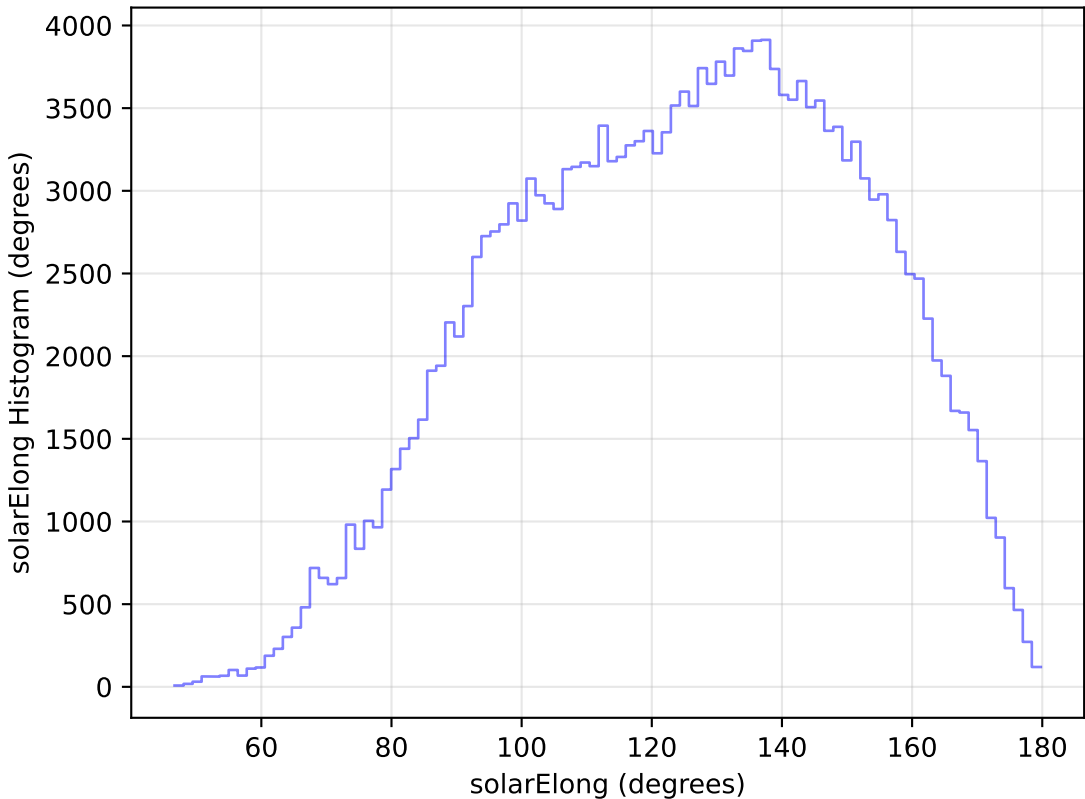
too_elab_heavy_r32_d3_gz_v3.4_10yrs WFD g band: solarElong Histogram
