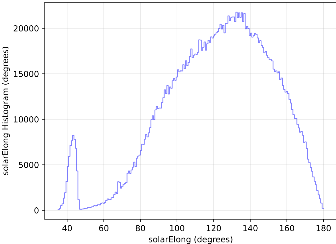
too_elab_heavy_r32_d3_gz_v3.4_10yrs WFD all bands: solarElong Histogram
