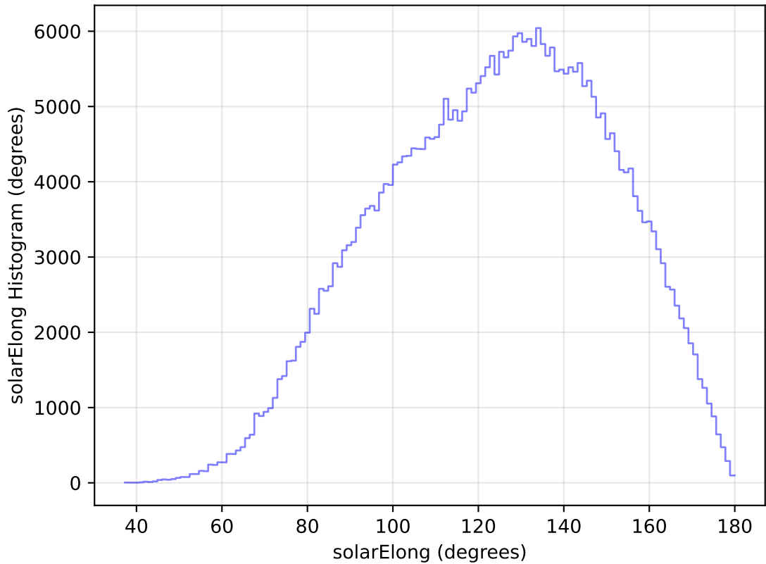
too_elab_heavy_r32_d3_gz_v3.4_10yrs All sky y band: solarElong Histogram
