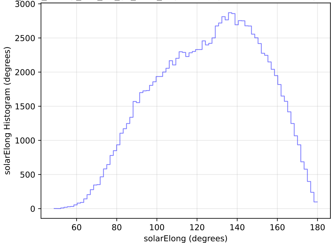
too_elab_heavy_r32_d3_gz_v3.4_10yrs All sky u band: solarElong Histogram
