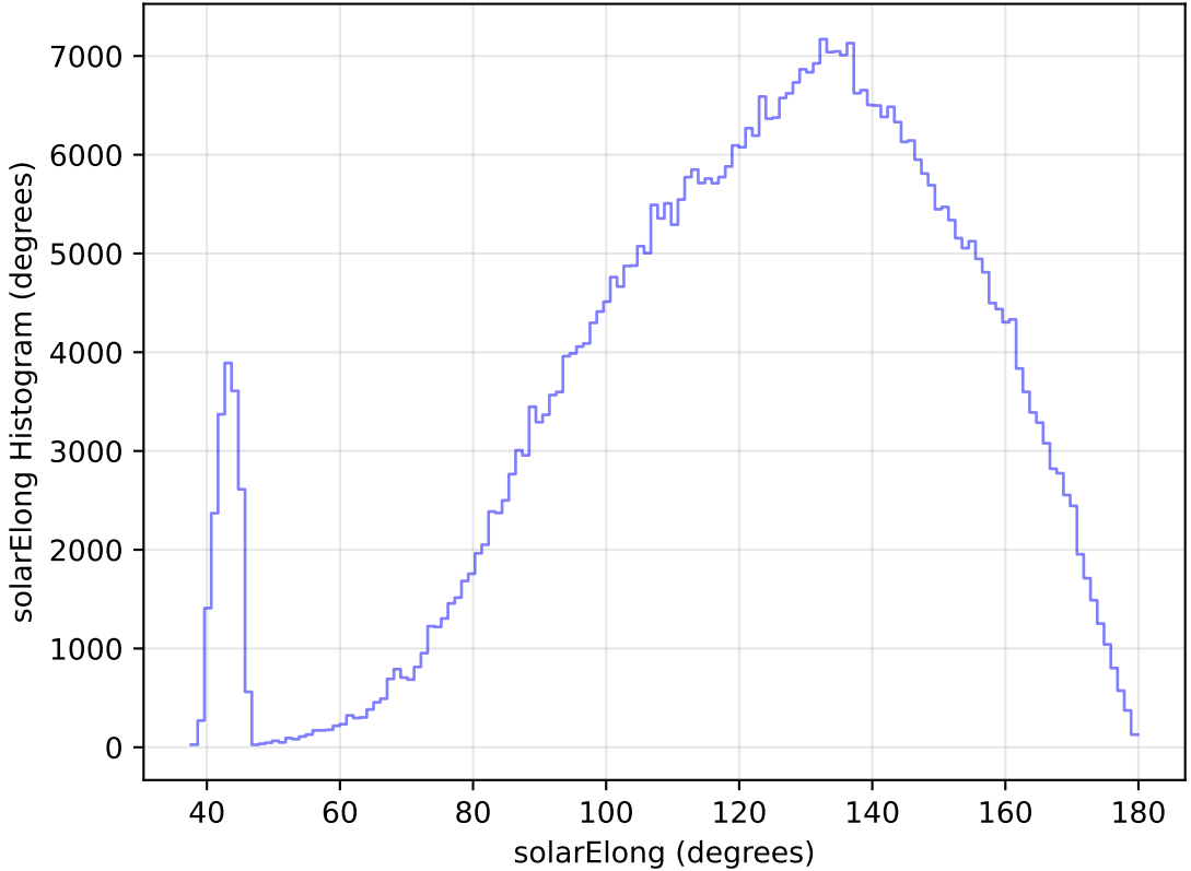
too_elab_heavy_r32_d3_gz_v3.4_10yrs All sky r band: solarElong Histogram
