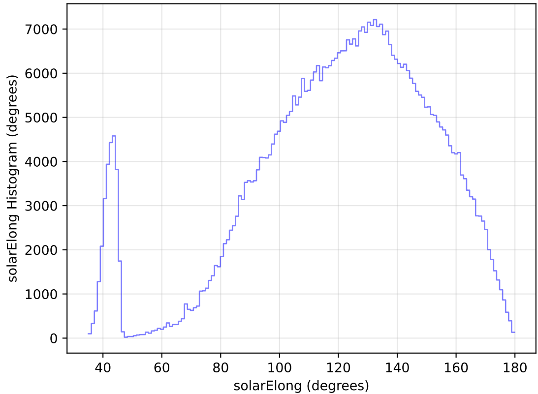
too_elab_heavy_r32_d3_gz_v3.4_10yrs All sky i band: solarElong Histogram
