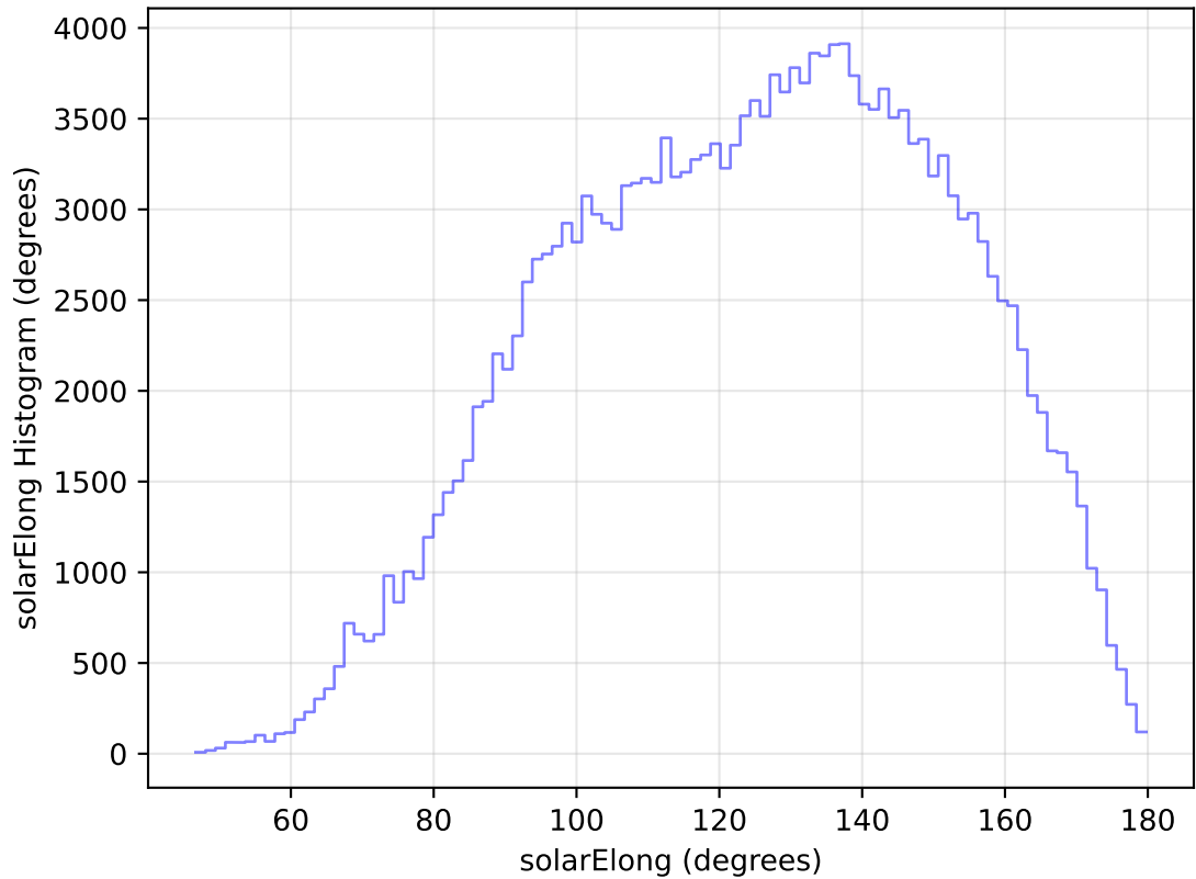
too_elab_heavy_r32_d3_gz_v3.4_10yrs All sky g band: solarElong Histogram
