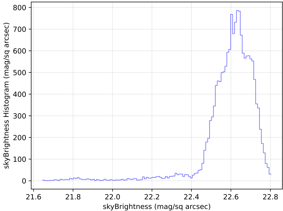
too_elab_heavy_r32_d3_gz_v3.4_10yrs Yr 1 u band: skyBrightness Histogram
