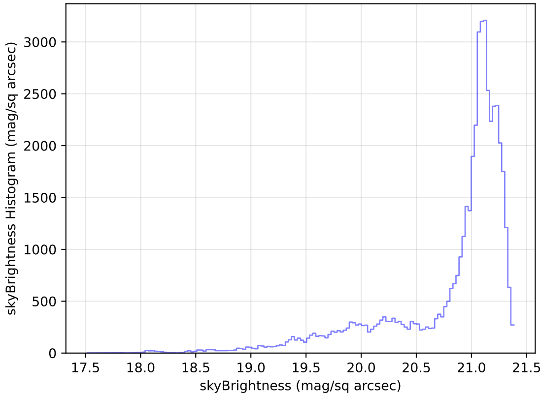
too_elab_heavy_r32_d3_gz_v3.4_10yrs Yr 1 r band: skyBrightness Histogram
