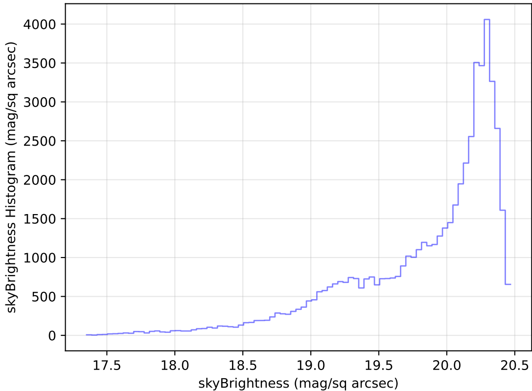
too_elab_heavy_r32_d3_gz_v3.4_10yrs Yr 1 i band: skyBrightness Histogram
