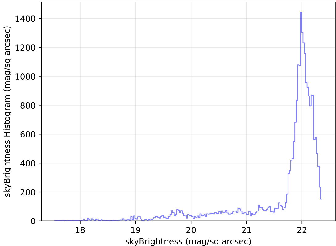
too_elab_heavy_r32_d3_gz_v3.4_10yrs Yr 1 g band: skyBrightness Histogram
