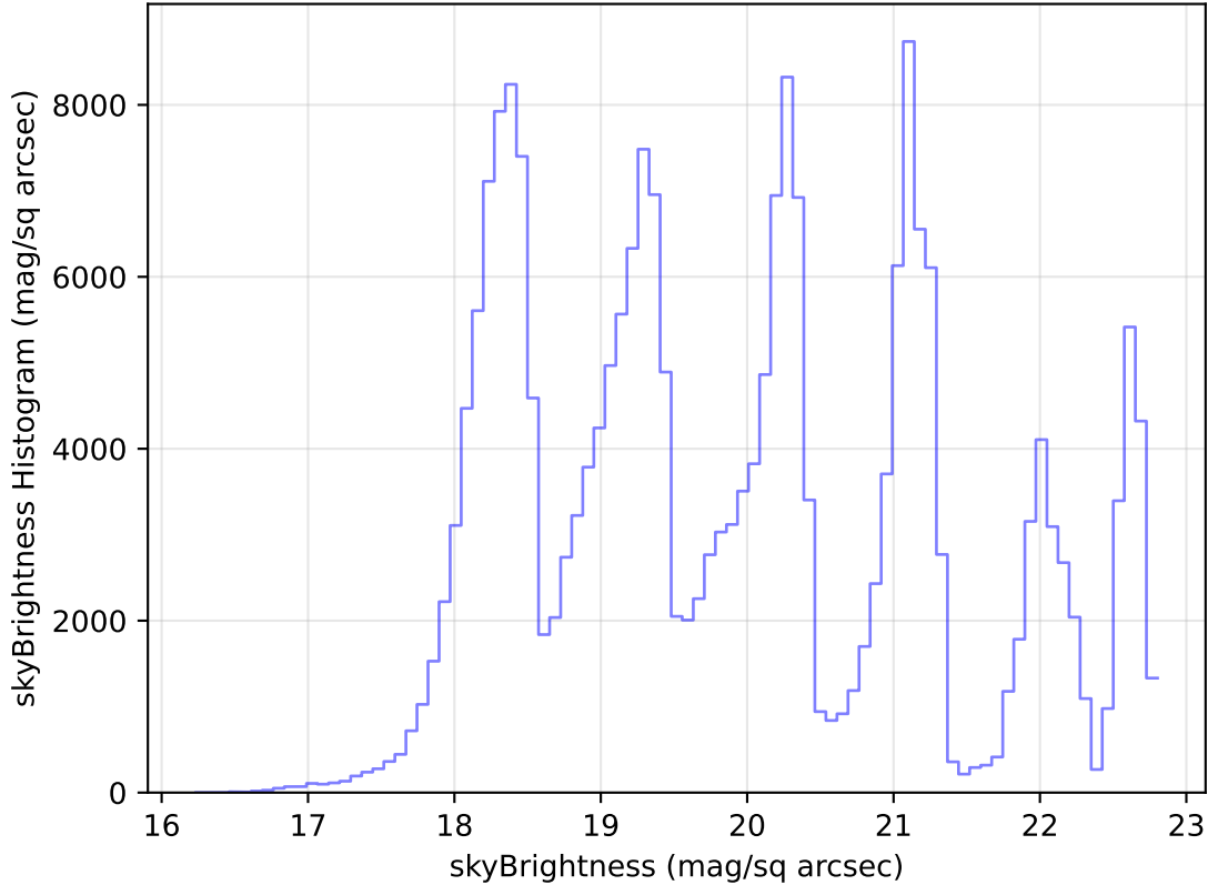
too_elab_heavy_r32_d3_gz_v3.4_10yrs Yr 1 all bands: skyBrightness Histogram
