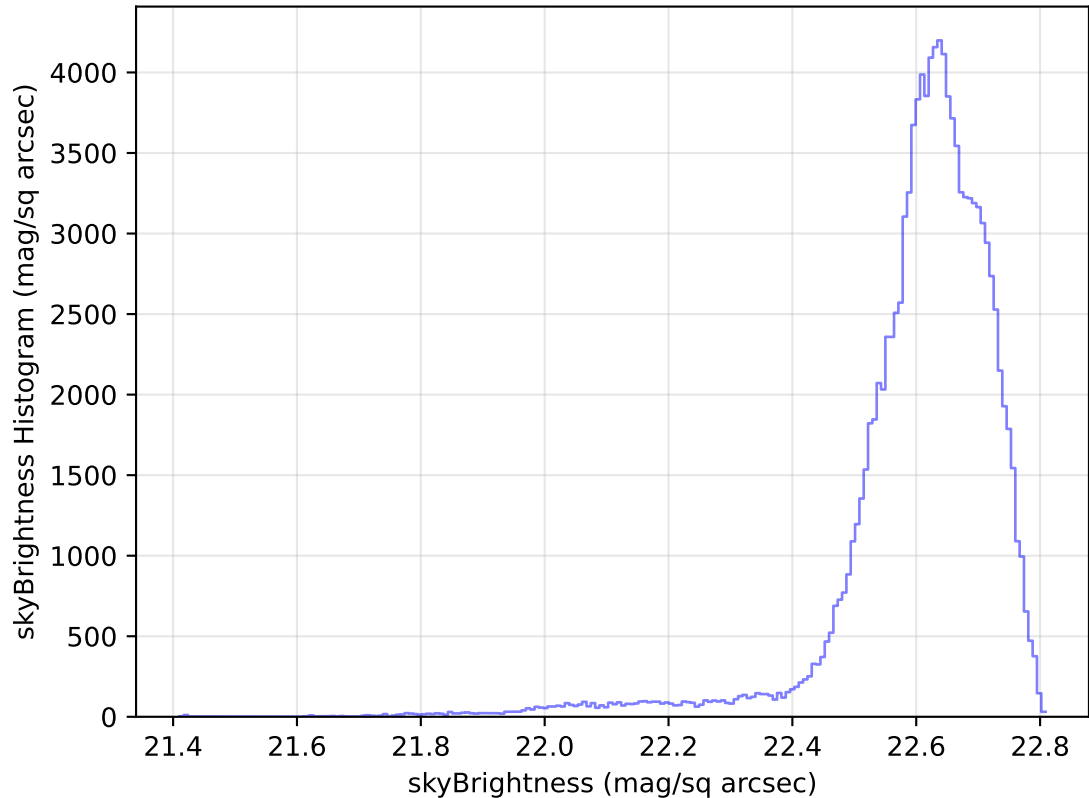
too_elab_heavy_r32_d3_gz_v3.4_10yrs WFD u band: skyBrightness Histogram
