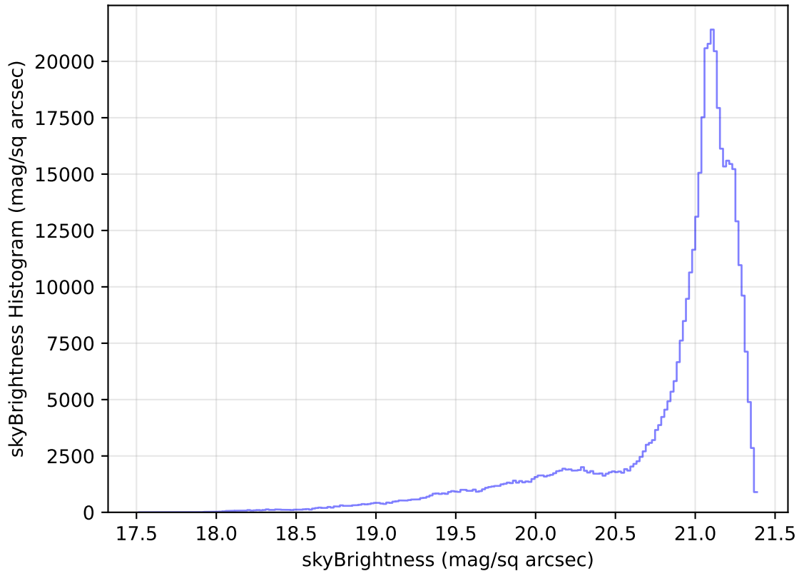
too_elab_heavy_r32_d3_gz_v3.4_10yrs WFD r band: skyBrightness Histogram
