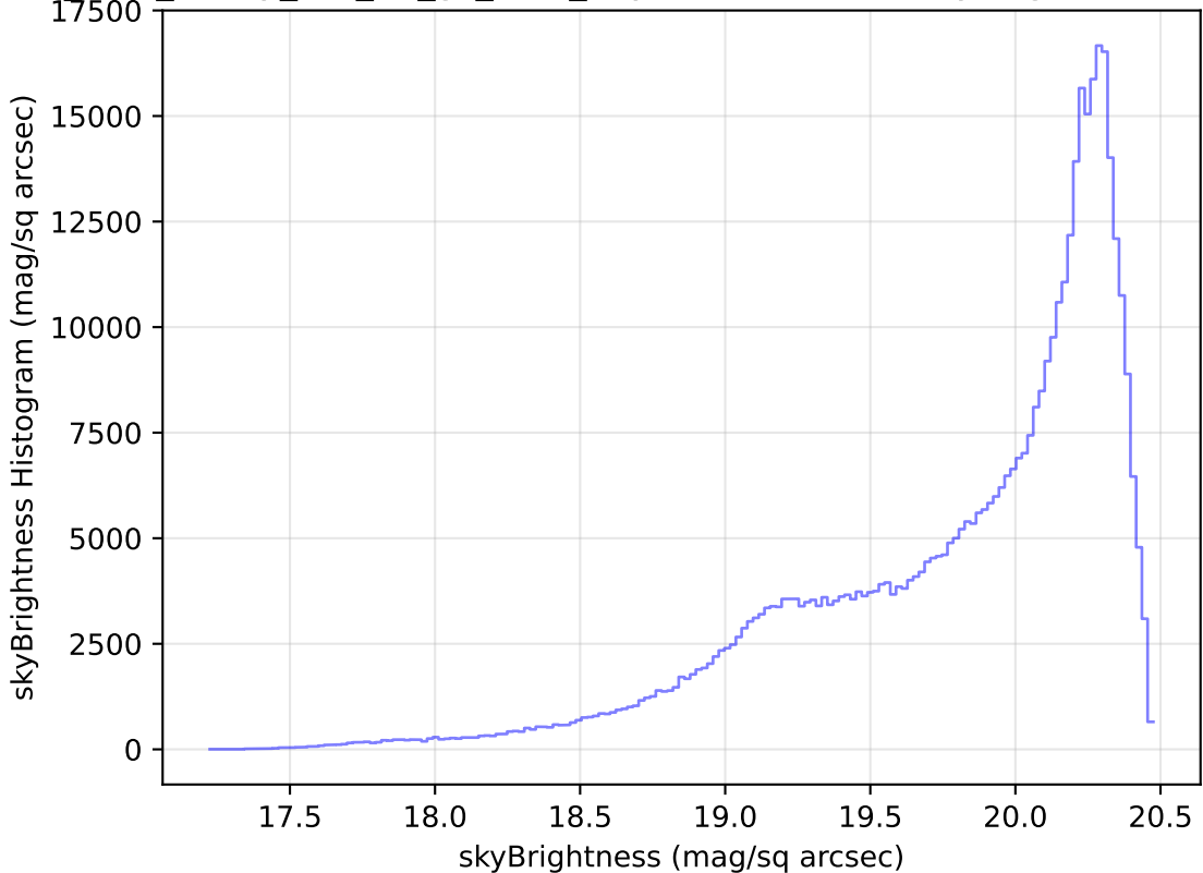
too_elab_heavy_r32_d3_gz_v3.4_10yrs WFD i band: skyBrightness Histogram
