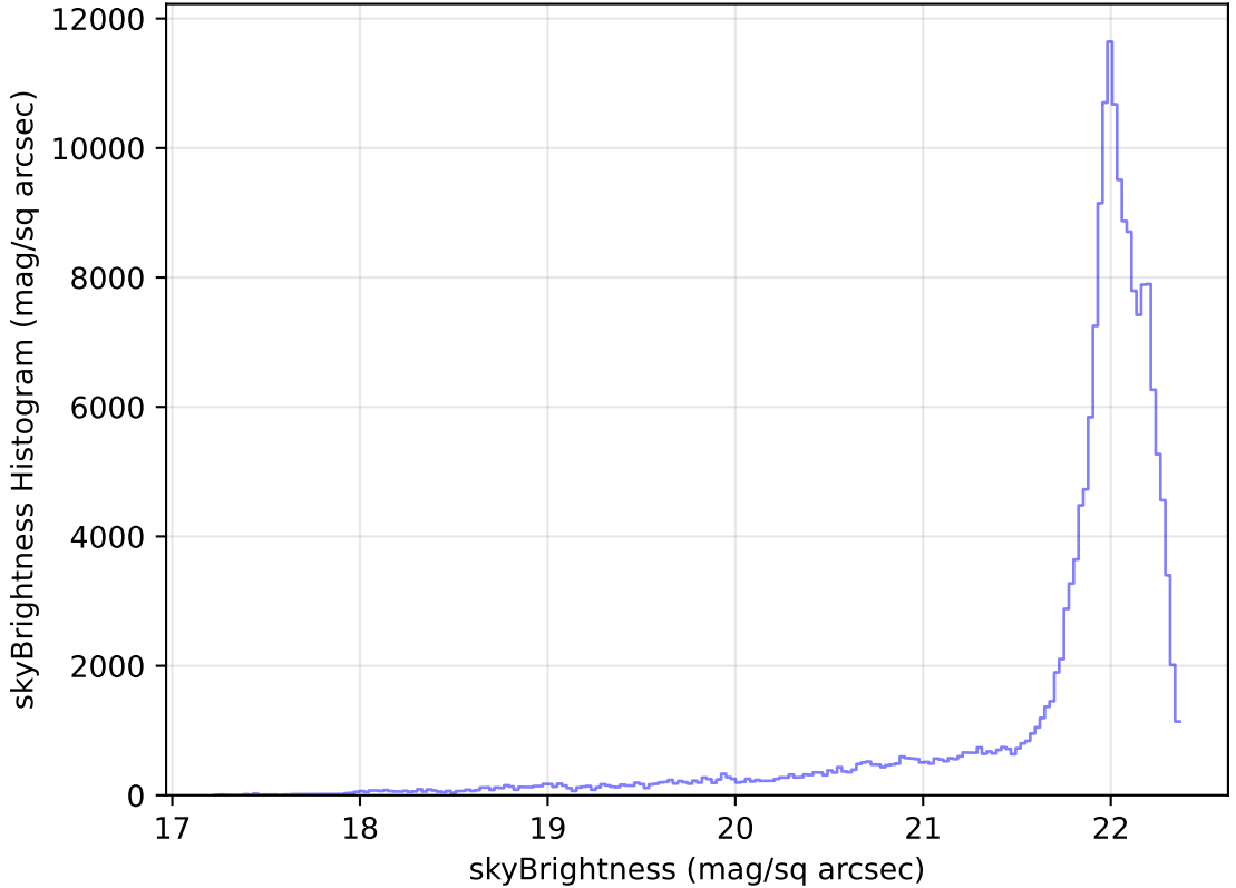
too_elab_heavy_r32_d3_gz_v3.4_10yrs WFD g band: skyBrightness Histogram
