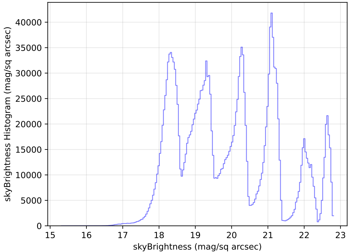
too_elab_heavy_r32_d3_gz_v3.4_10yrs WFD all bands: skyBrightness Histogram
