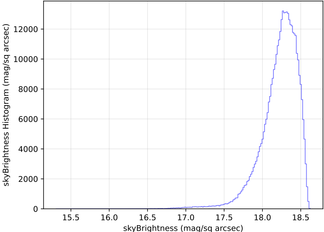
too_elab_heavy_r32_d3_gz_v3.4_10yrs All sky y band: skyBrightness Histogram
