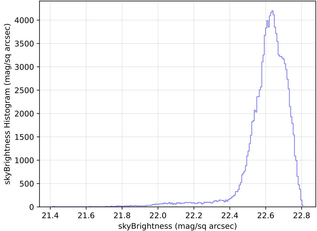
too_elab_heavy_r32_d3_gz_v3.4_10yrs All sky u band: skyBrightness Histogram
