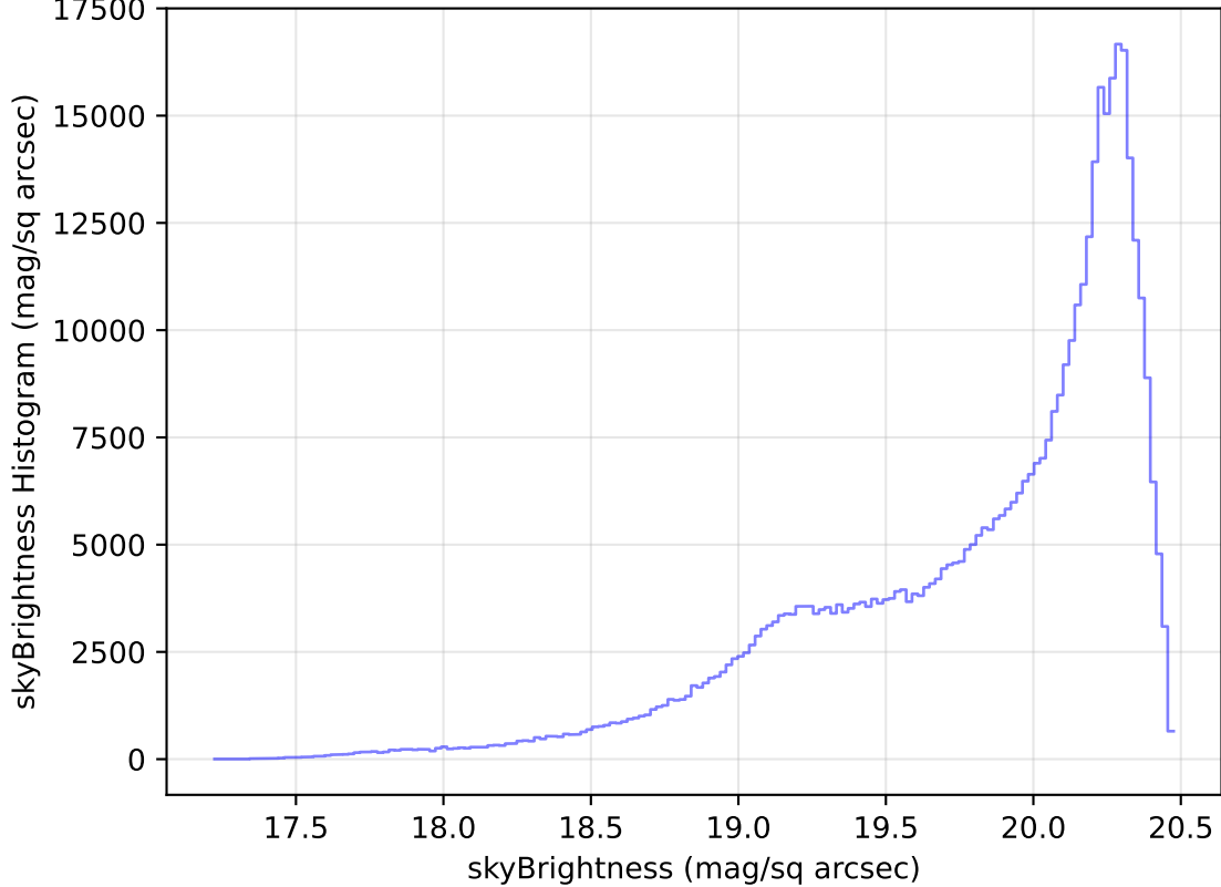
too_elab_heavy_r32_d3_gz_v3.4_10yrs All sky i band: skyBrightness Histogram
