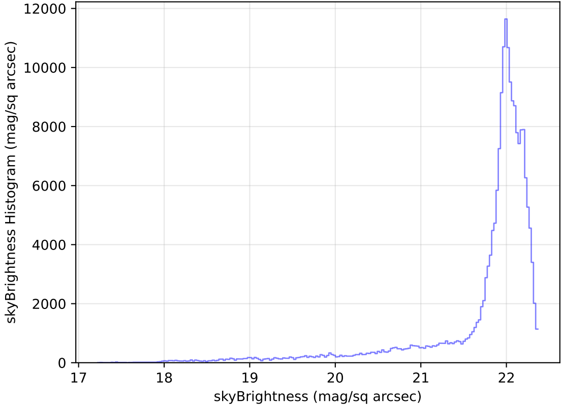
too_elab_heavy_r32_d3_gz_v3.4_10yrs All sky g band: skyBrightness Histogram
