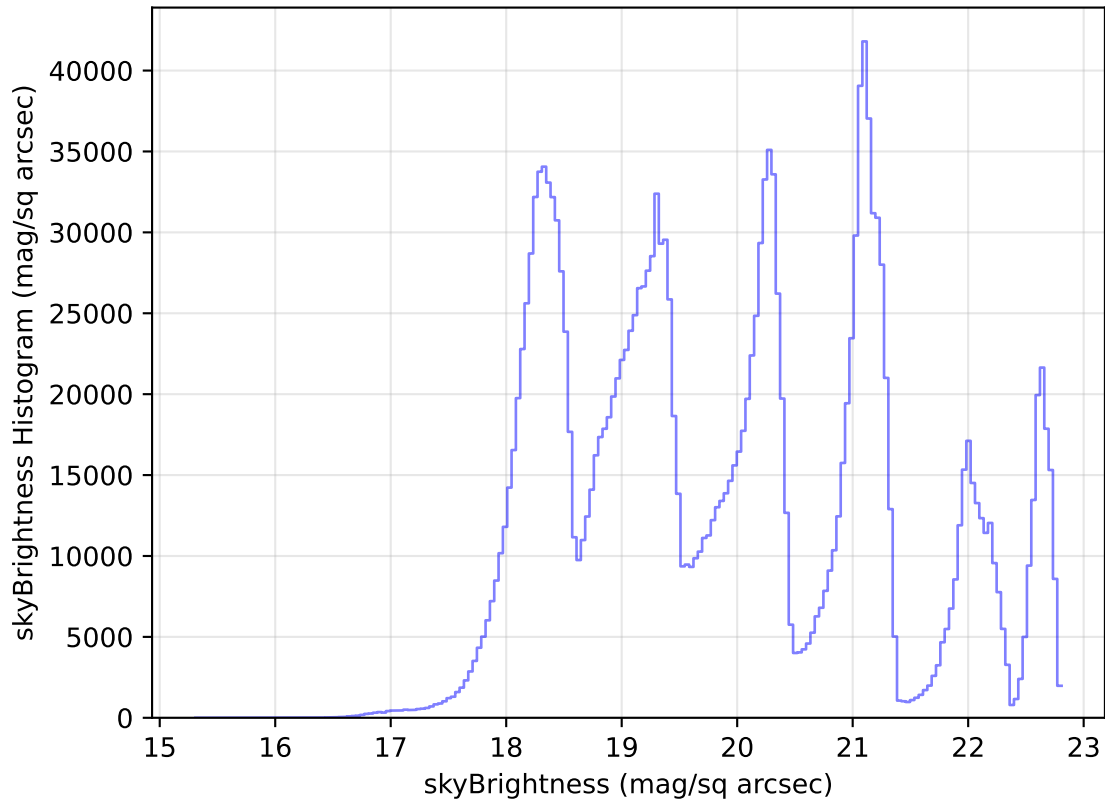
too_elab_heavy_r32_d3_gz_v3.4_10yrs All sky all bands: skyBrightness Histogram
