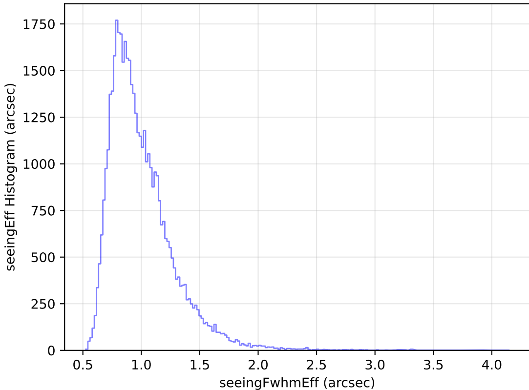
too_elab_heavy_r32_d3_gz_v3.4_10yrs Yr 1 z band: seeingEff Histogram
