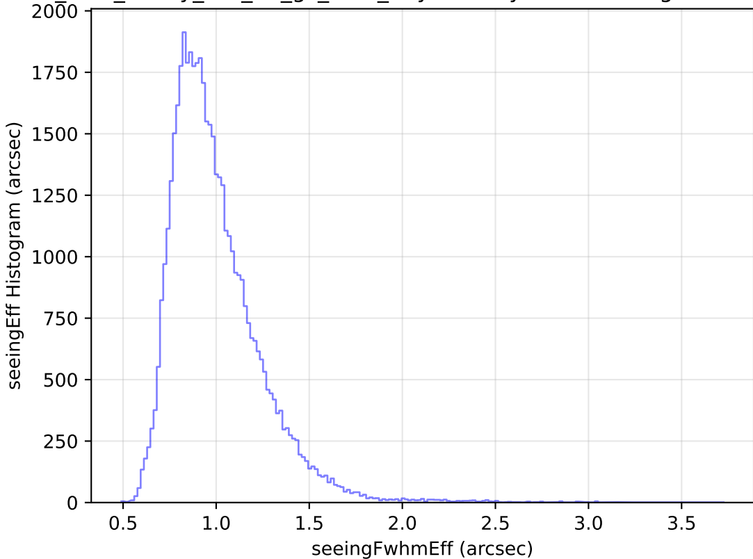
too_elab_heavy_r32_d3_gz_v3.4_10yrs Yr 1 y band: seeingEff Histogram
