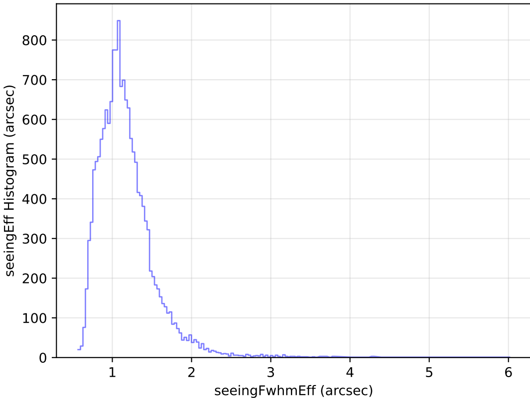
too_elab_heavy_r32_d3_gz_v3.4_10yrs Yr 1 u band: seeingEff Histogram
