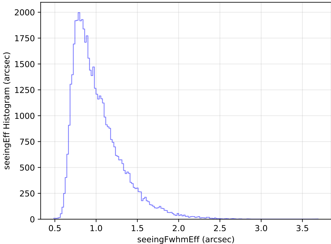
too_elab_heavy_r32_d3_gz_v3.4_10yrs Yr 1 r band: seeingEff Histogram
