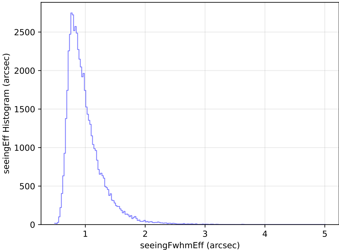
too_elab_heavy_r32_d3_gz_v3.4_10yrs Yr 1 i band: seeingEff Histogram
