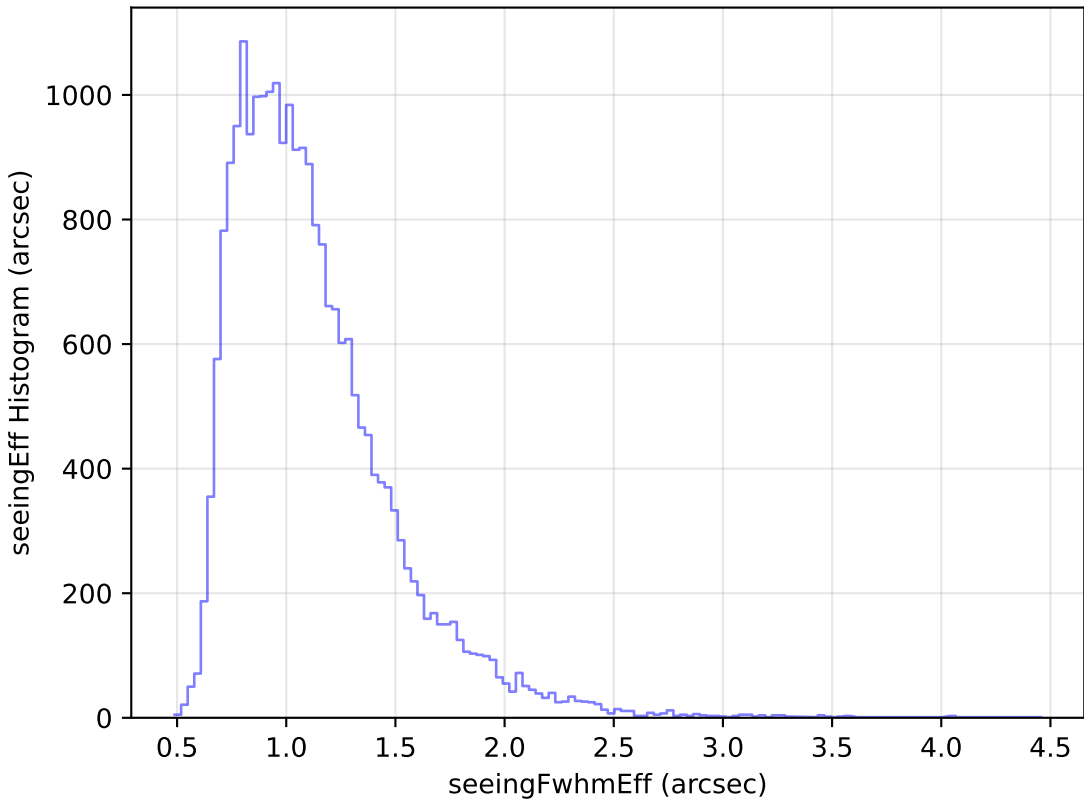
too_elab_heavy_r32_d3_gz_v3.4_10yrs Yr 1 g band: seeingEff Histogram
