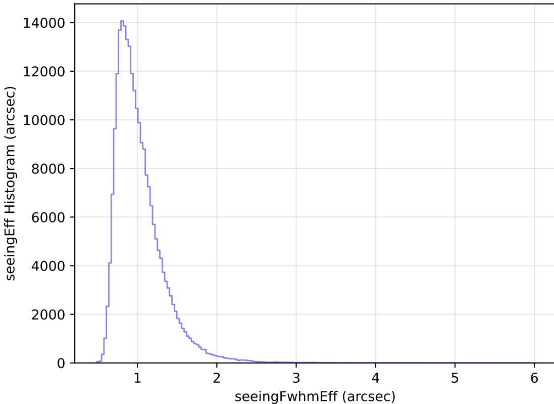
too_elab_heavy_r32_d3_gz_v3.4_10yrs Yr 1 all bands: seeingEff Histogram
