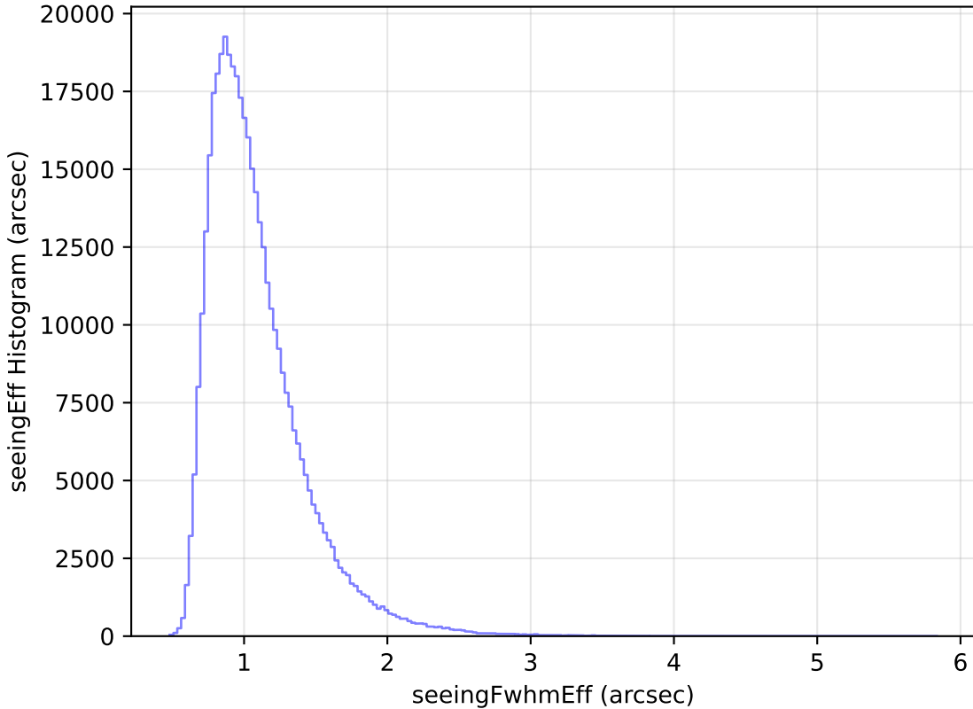
too_elab_heavy_r32_d3_gz_v3.4_10yrs WFD z band: seeingEff Histogram
