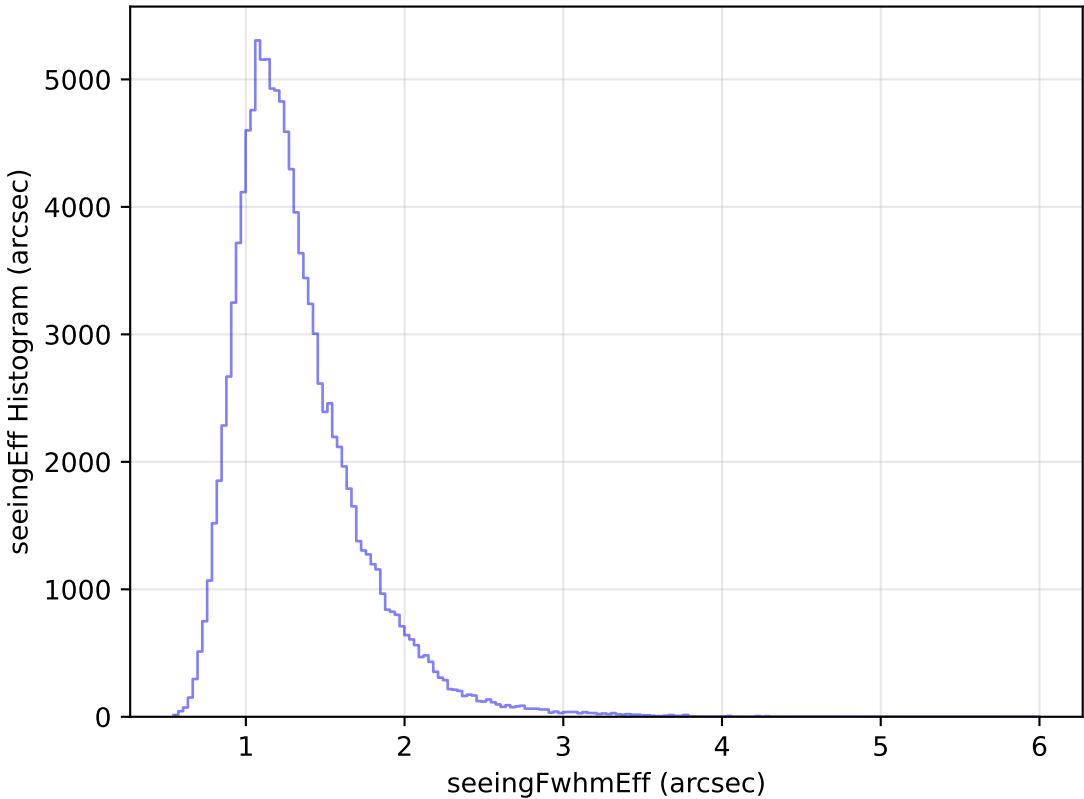
too_elab_heavy_r32_d3_gz_v3.4_10yrs WFD u band: seeingEff Histogram
