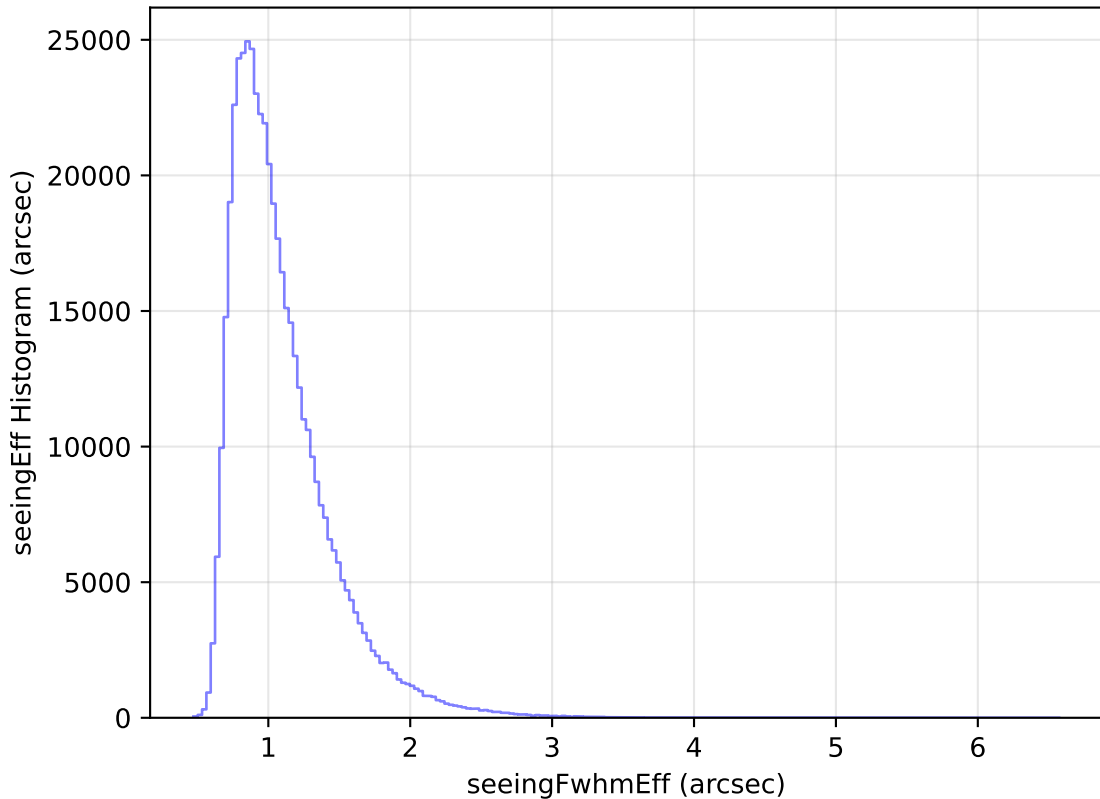
too_elab_heavy_r32_d3_gz_v3.4_10yrs WFD i band: seeingEff Histogram
