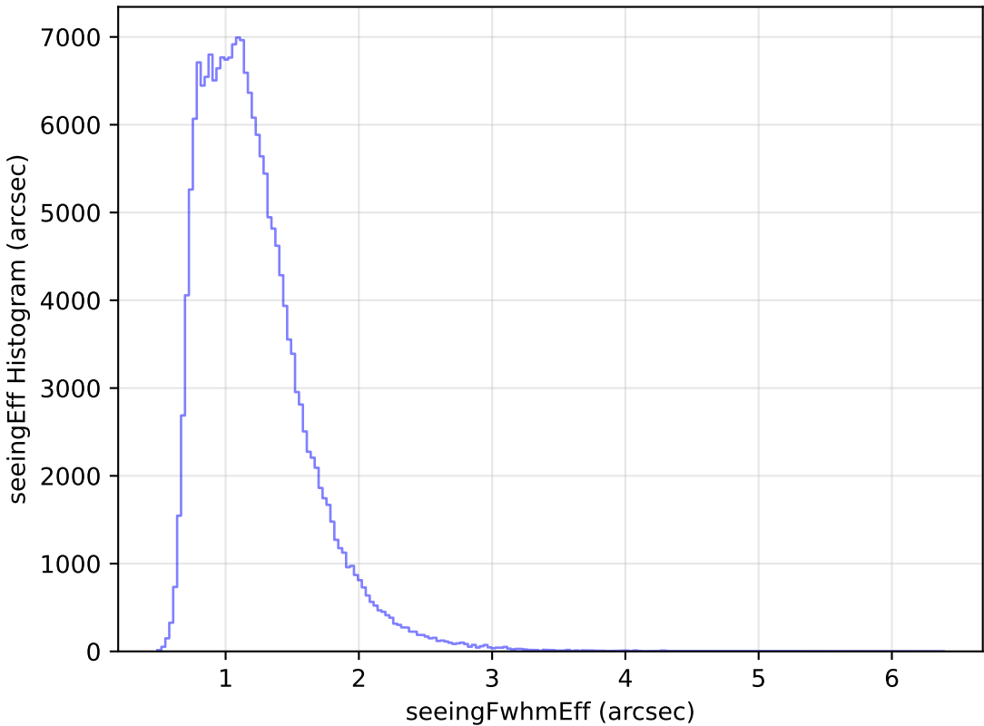
too_elab_heavy_r32_d3_gz_v3.4_10yrs WFD g band: seeingEff Histogram
