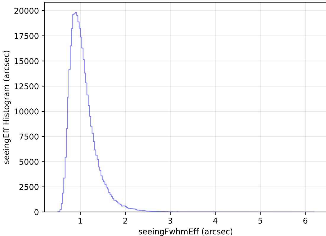
too_elab_heavy_r32_d3_gz_v3.4_10yrs All sky y band: seeingEff Histogram
