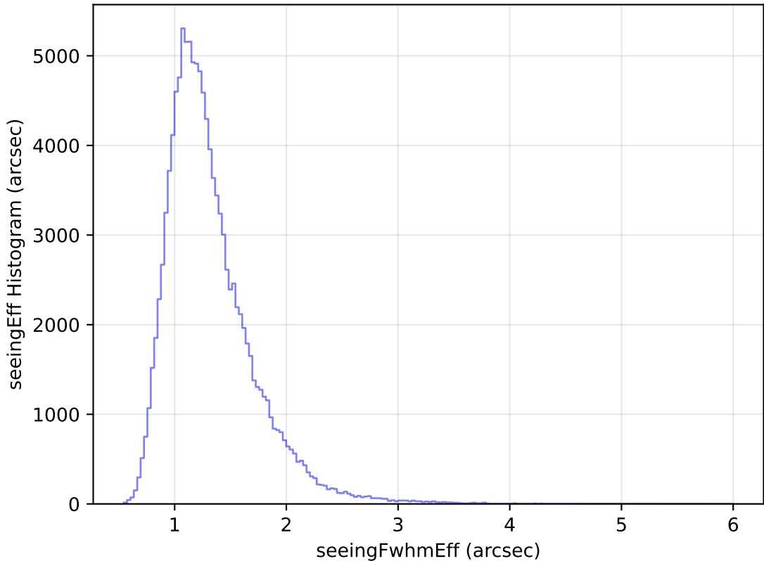
too_elab_heavy_r32_d3_gz_v3.4_10yrs All sky u band: seeingEff Histogram
