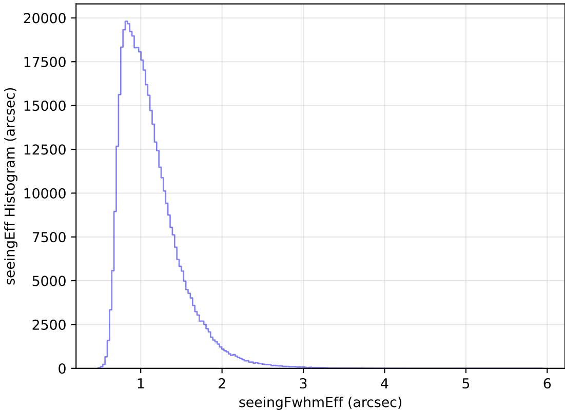
too_elab_heavy_r32_d3_gz_v3.4_10yrs All sky r band: seeingEff Histogram
