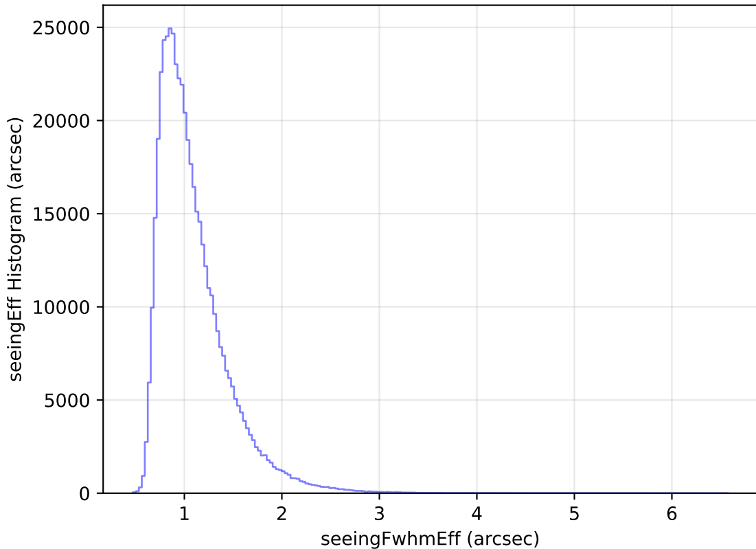
too_elab_heavy_r32_d3_gz_v3.4_10yrs All sky i band: seeingEff Histogram
