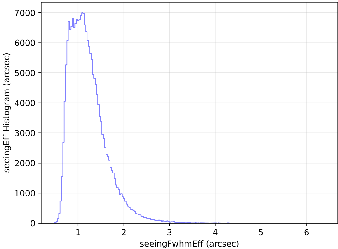
too_elab_heavy_r32_d3_gz_v3.4_10yrs All sky g band: seeingEff Histogram
