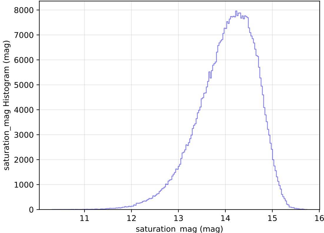
too_elab_heavy_r32_d3_gz_v3.4_10yrs WFD z band: saturation_mag Histogram
