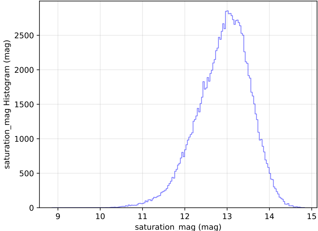
too_elab_heavy_r32_d3_gz_v3.4_10yrs WFD u band: saturation_mag Histogram
