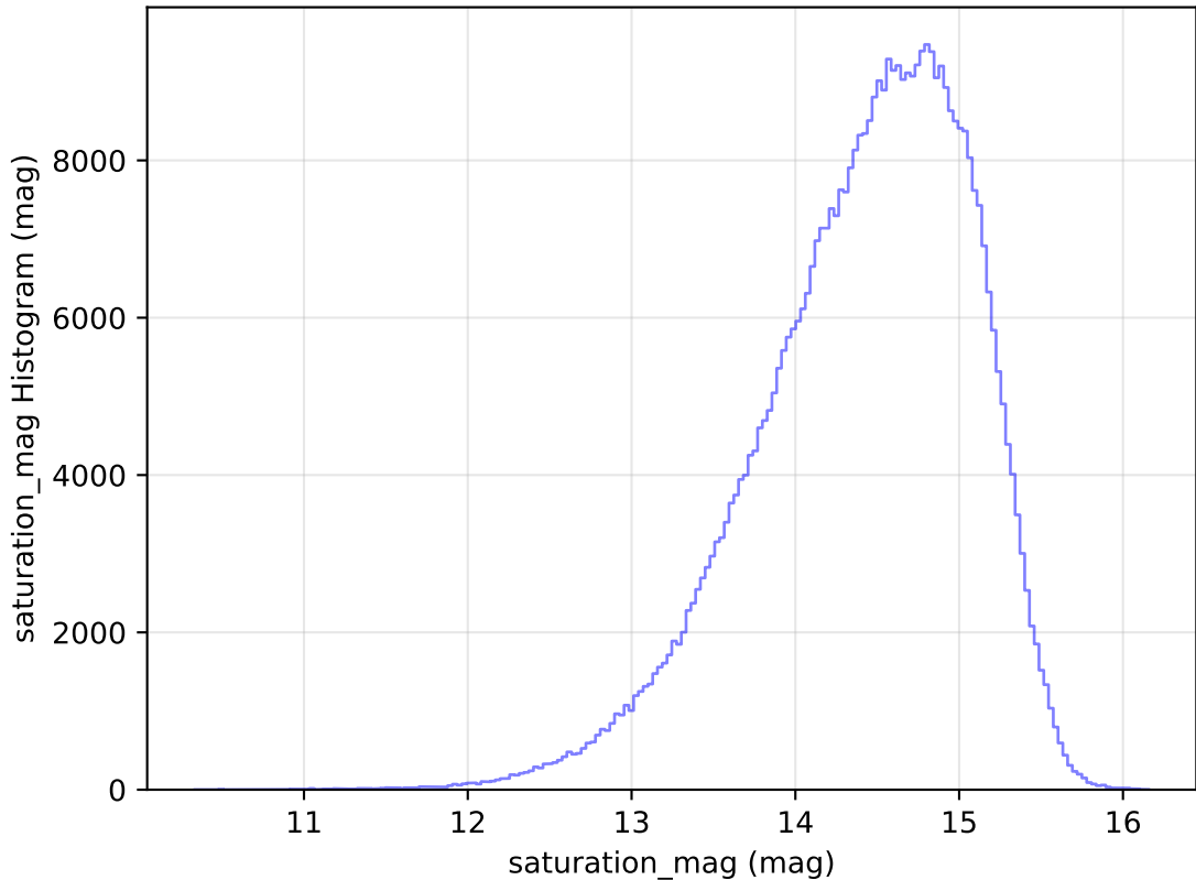
too_elab_heavy_r32_d3_gz_v3.4_10yrs WFD i band: saturation_mag Histogram
