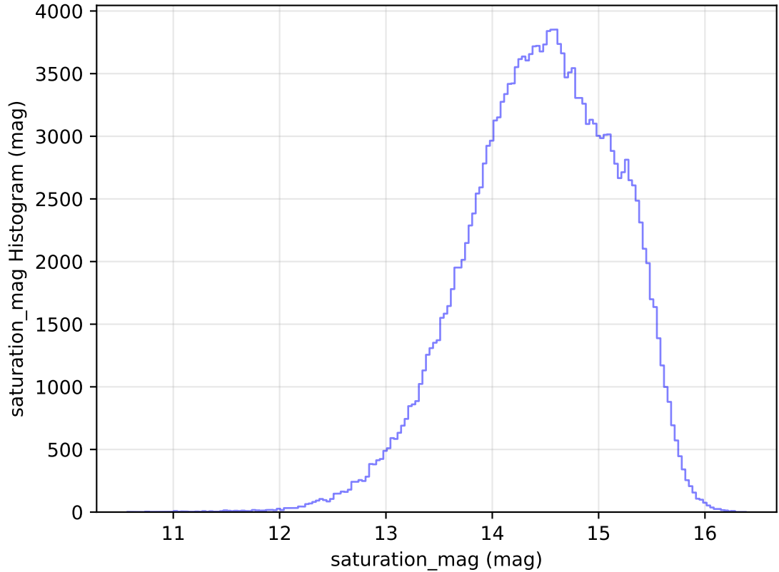
too_elab_heavy_r32_d3_gz_v3.4_10yrs WFD g band: saturation_mag Histogram
