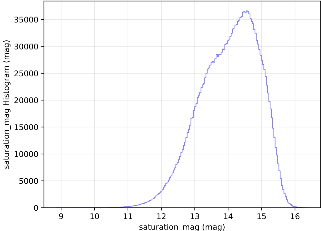
too_elab_heavy_r32_d3_gz_v3.4_10yrs WFD all bands: saturation_mag Histogram
