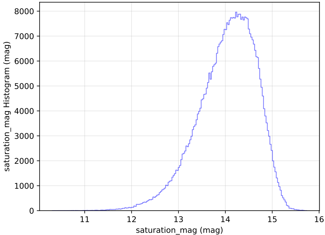
too_elab_heavy_r32_d3_gz_v3.4_10yrs All sky z band: saturation_mag Histogram
