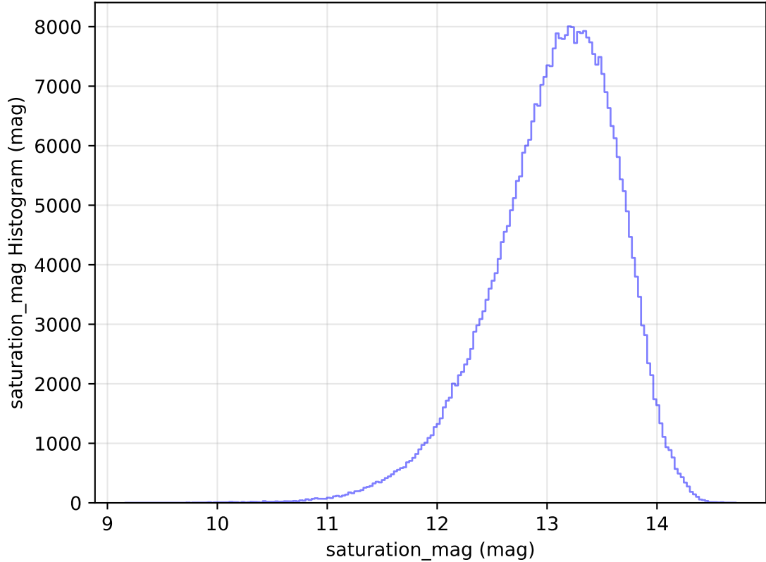
too_elab_heavy_r32_d3_gz_v3.4_10yrs All sky y band: saturation_mag Histogram
