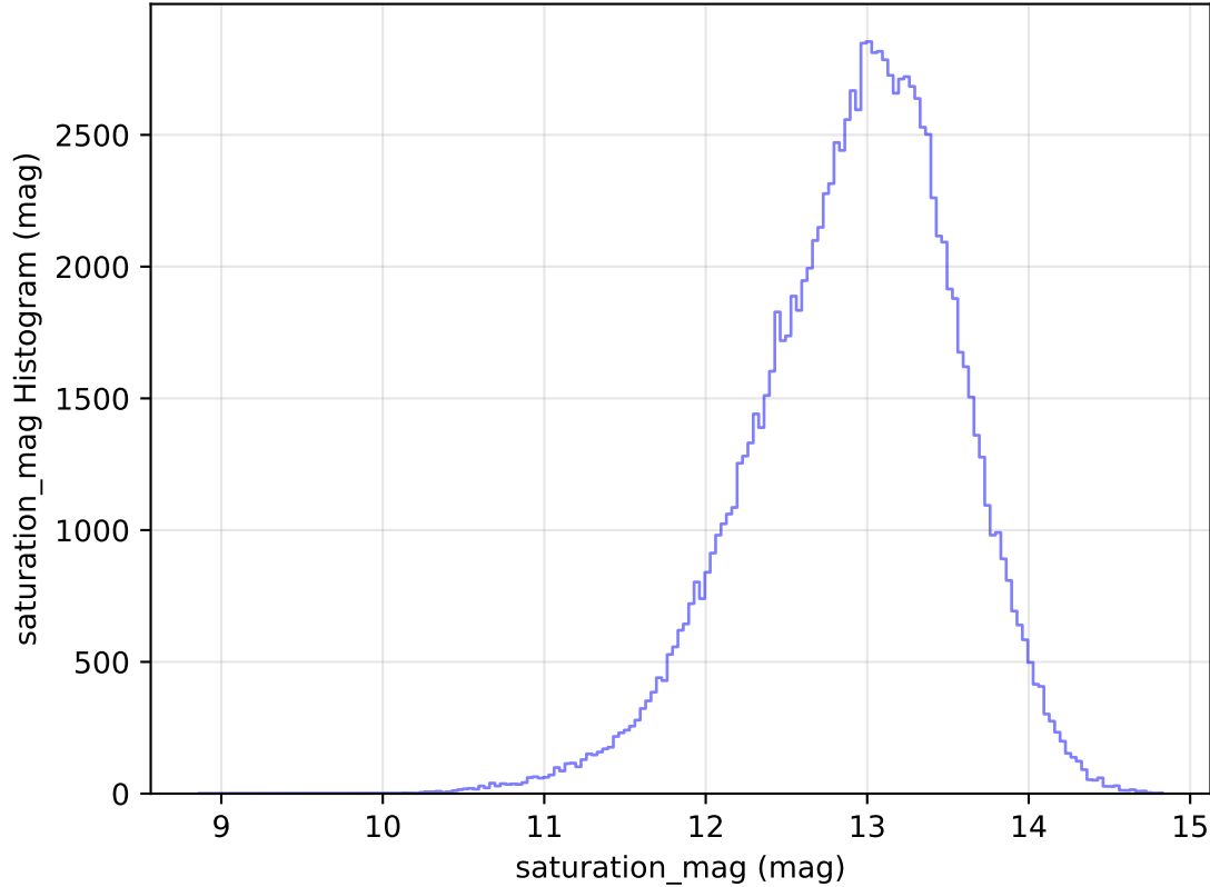
too_elab_heavy_r32_d3_gz_v3.4_10yrs All sky u band: saturation_mag Histogram
